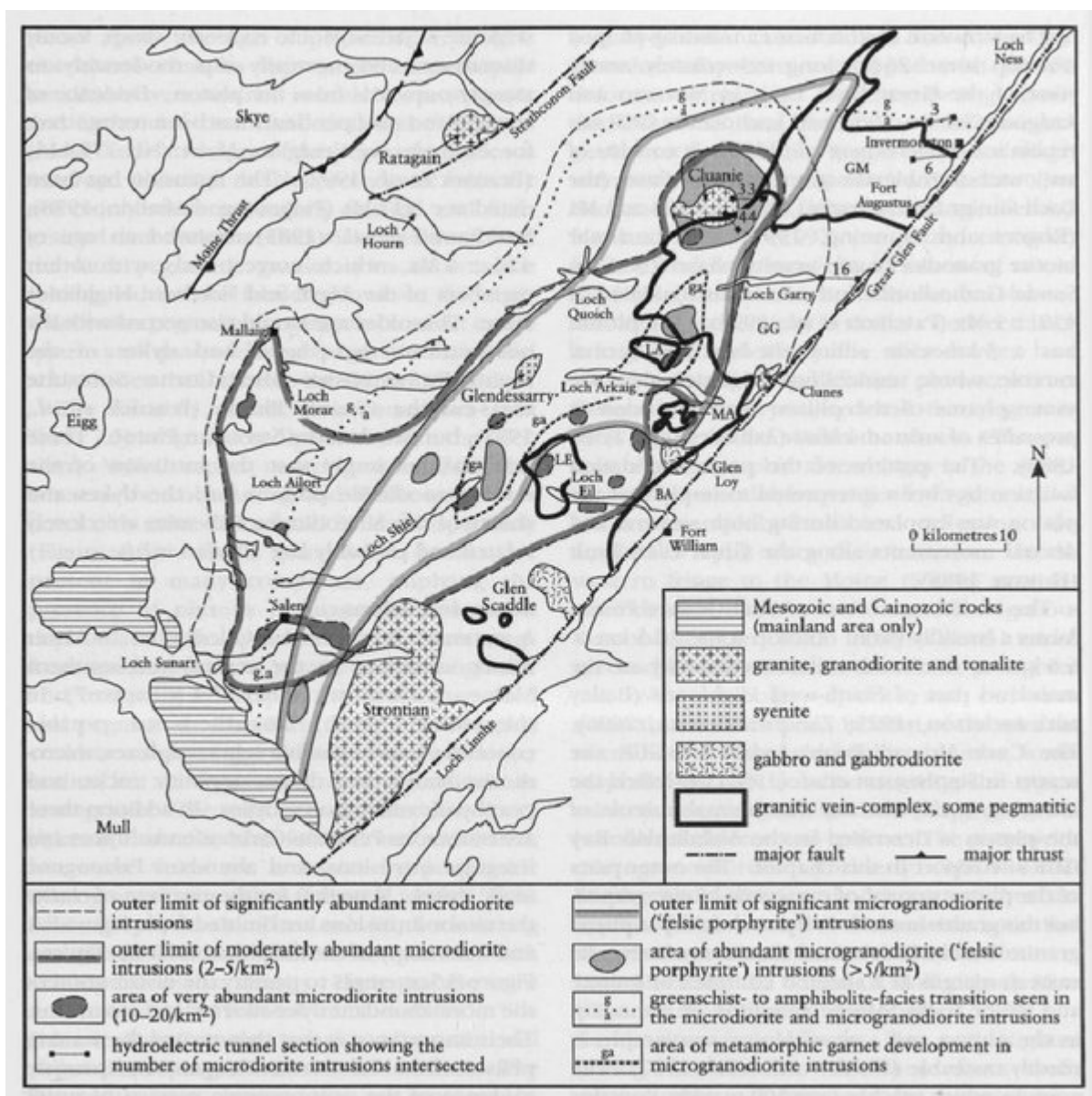
(Figure 8.5) Map showing the Caledonian major and minor intrusions. Granitic vein-complexes: Ba — Banavie; GG — Glen Garry; GM — Glen Moriston; LA — Loch Arkatig; LE — Loch Eil; MA — Maine.
