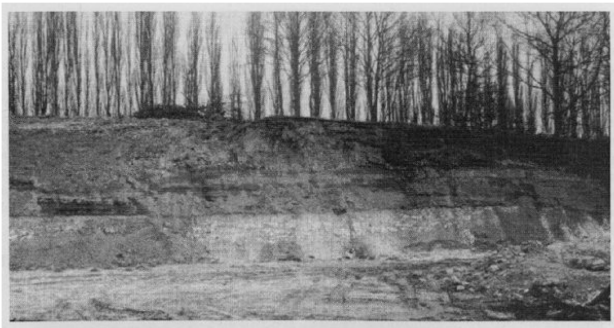
(Figure 4.3) Pincent's Kiln, Theale, Berkshire, showing the Palaeogene (Lambeth Group) resting unconformably on the Upper Cretaceous Chalk. (Photograph courtesy R. Goldring, who obtained this picture in 1979 after the site had been re-excavated by NCC.)
