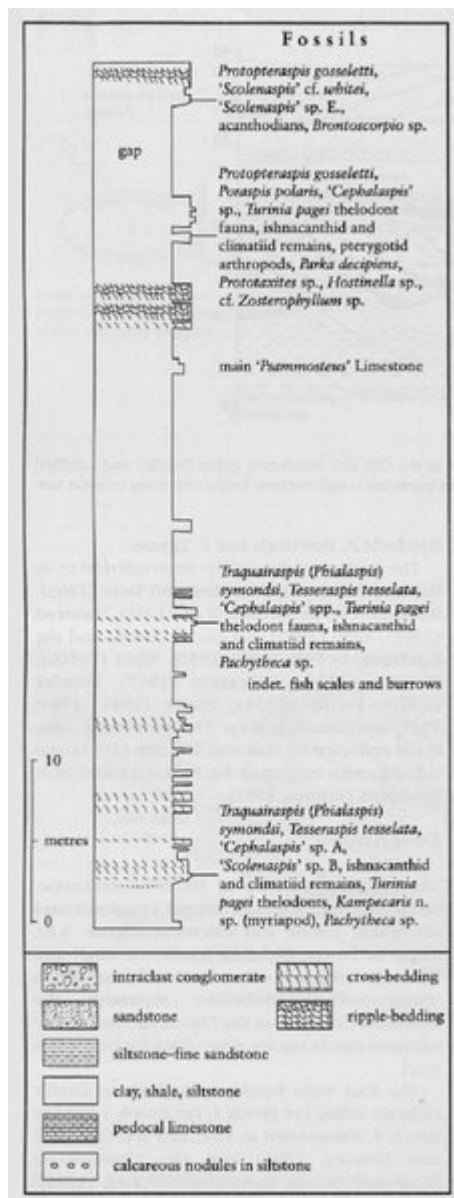
(Figure 4.8) Stratigraphical section in The Devil's Hole (after M.A. Rowlands, MS). The base of the Main ' Psammosteus ' Limestone is mapped as the base of the Ditton Group, which has predominantly pteraspigid faunas.
