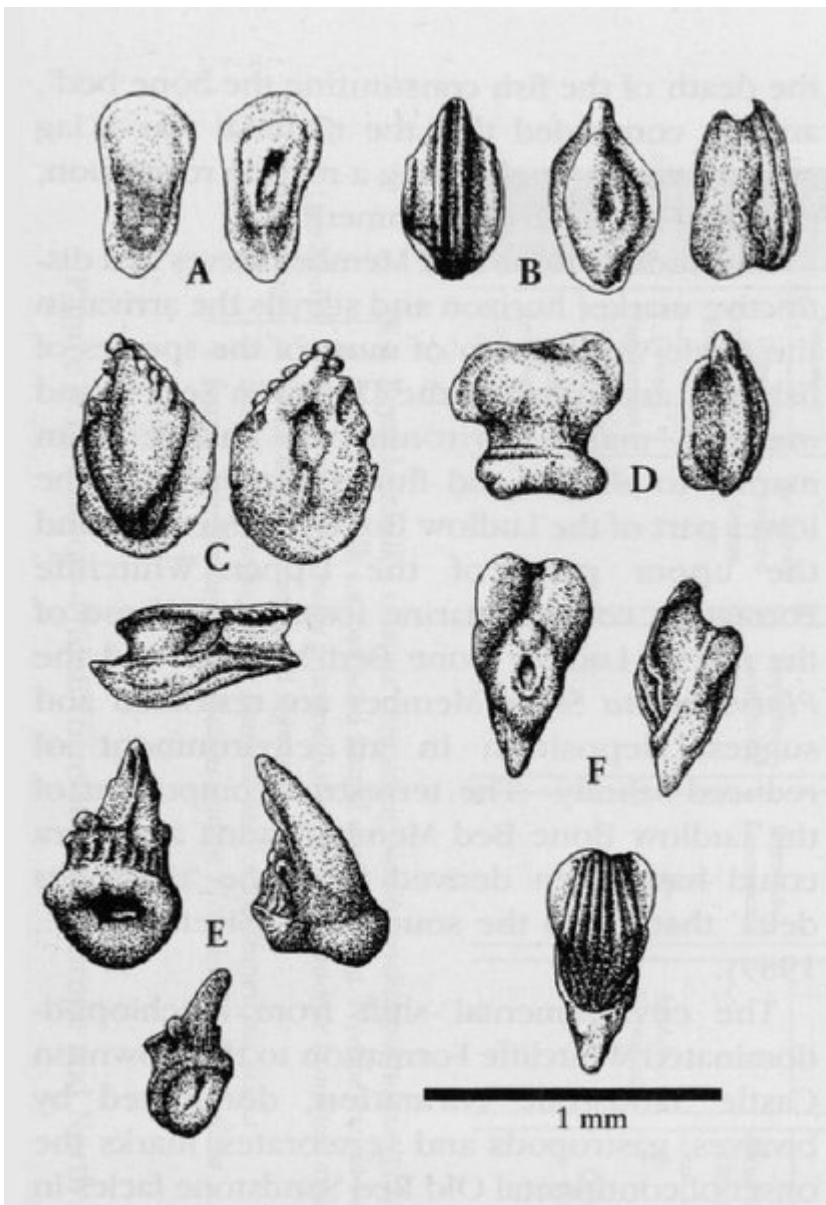
(Figure 3.11) Thelodonts from the Ludlow Bone Bed (after Turner 1973). (A) Thedolus parvidens ; (B) Thelodus bicostatus ; (C) Loganellia ludlowiensis head scale; (D) Thedolus pugniformis ; (E) Thelodus parvidens? ; (F) Thelodus trilobatus .
