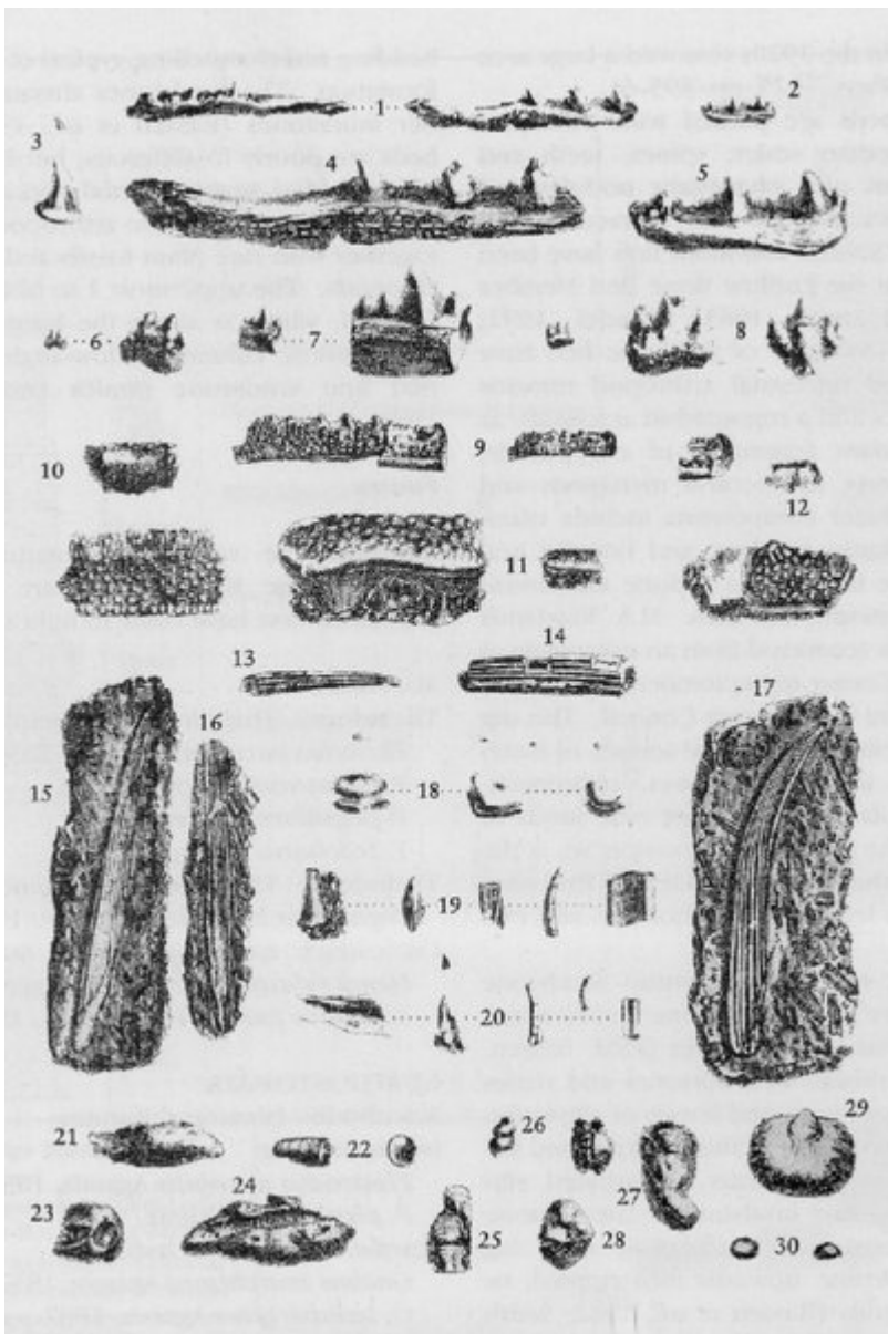
(Figure 3.10) Fossils from the Ludlow Bone Bed illustrated in a plate from Murchison's Siluria (1872). 1–8, Plectrodus mirabilis , fragments of jaws; 9–12, P. pustuliferus , fragments of jaws; 13, 14, Onchus murchisoni , fin spines; 15–17, O. trenuistriatus , fin spines; 18, Thelodus parvidens , denticles; 19–20, indeterminate fragments; 21–28, coprolites containing invertebrate fragments; 29, Orthis lunata Sowerby; 30, Pachtheca sphaerica . All approximately natural size.
