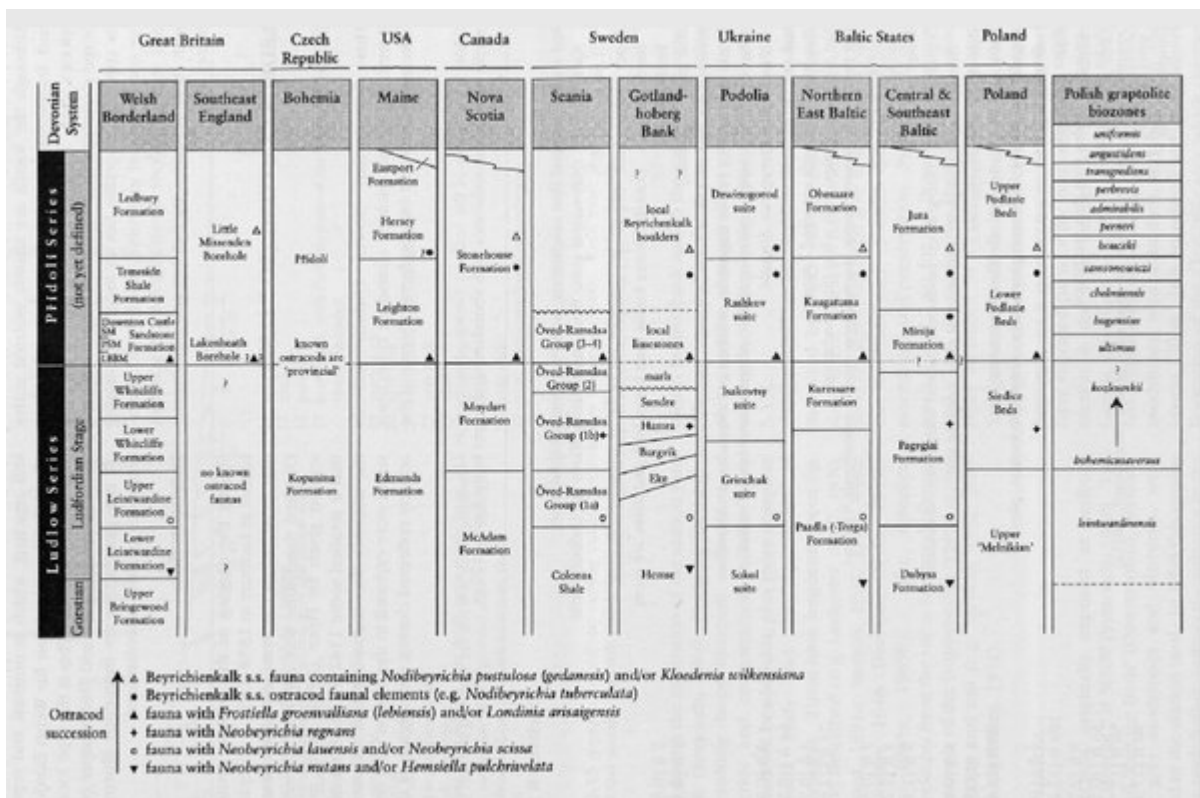
(Figure 3.12) Ludlow- Píldol correlation for Europe and North America. Vertical columns not drawn to scale (after Siveter et al., 1989).
