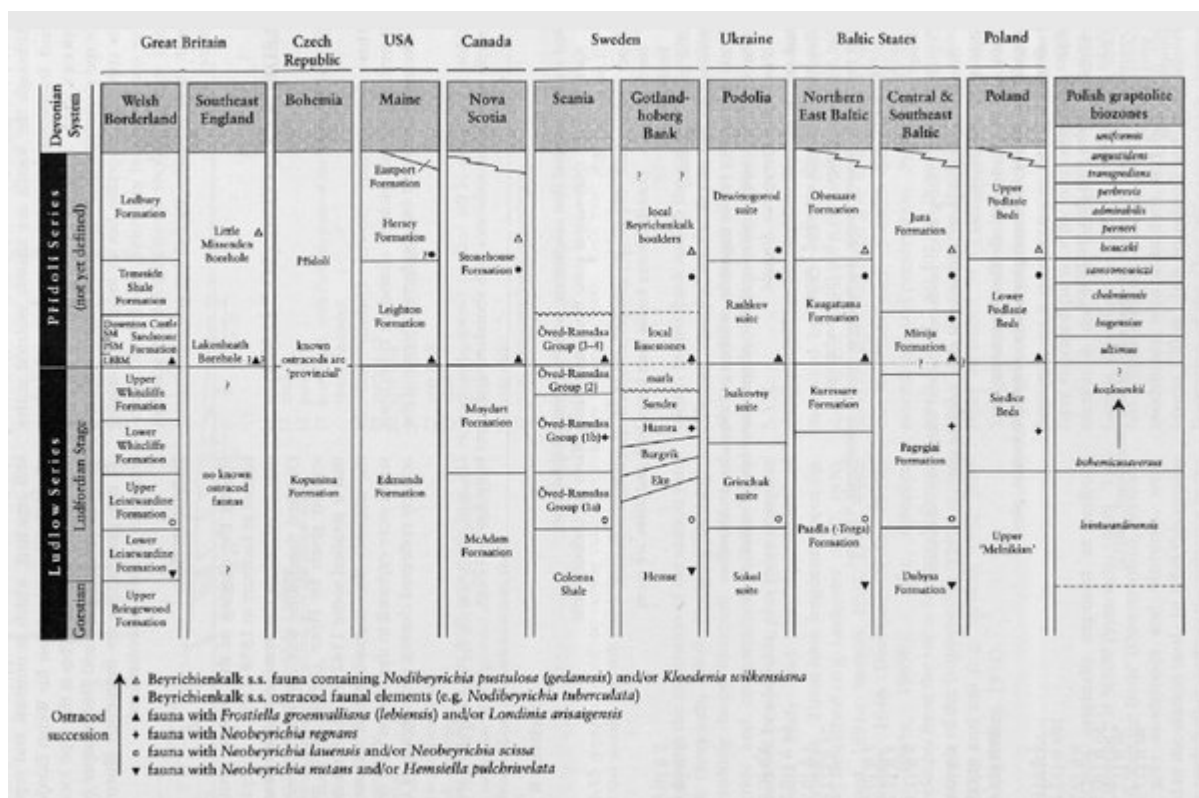
(Figure 3.12) Ludlow- Pridoli correlation for Europe and North America. Vertical columns not drawn to scale (after Siveter et al., 1989).
