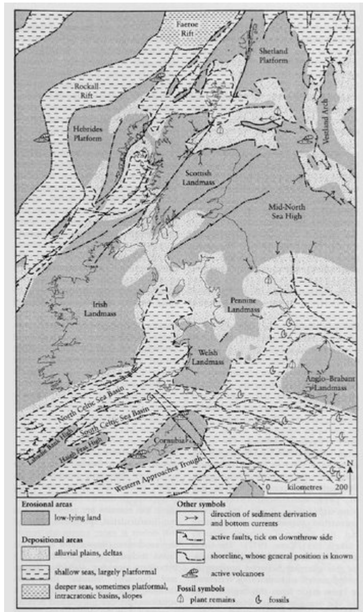
(Figure 12.13) Palaeogeography of the Middle Jurassic (after Bradshaw et al., 1992).
