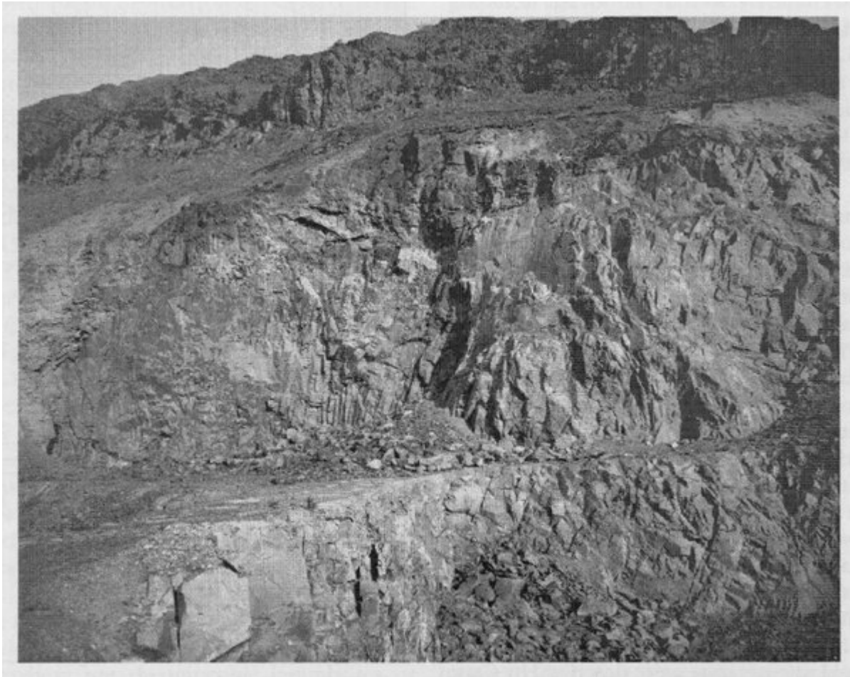
(Figure 4.32) Bramcrag Quarry: the Threlkeld microgranite is overlain by lavas and volcaniclastic sedimentary rocks of the basal part of the Borrowdale Volcanic Group. The contact slopes from top right to lower left. (Photo: BGS no. L2041.)
