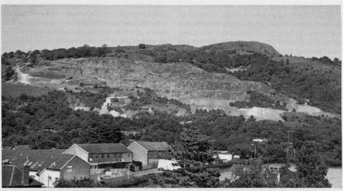
(Figure 6.29) Llanelwedd quarries, Builth Wells, viewed from the south. Westerly-dipping basic lavas, belonging to the Builth Volcanic Group, comprise much of the quarry area. Other volcanic units form the prominent features in the hills behind the quarry, the slack ground being eroded into softer shales. (Photo: R.E. Bevins.)
