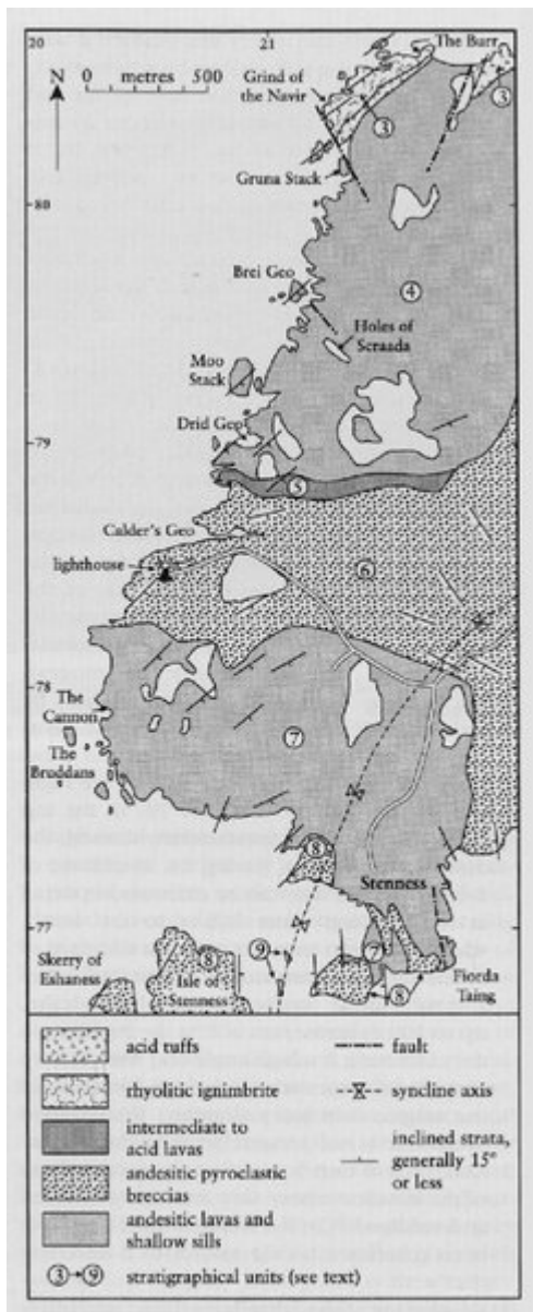
(Figure 9.47) Map of the Eshaness coast, adapted from Geological Survey 1:10 560 sheets Shetland 19 and Shetland 23 (1959).
