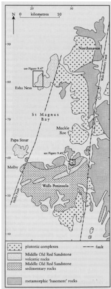
(Figure 9.46) Location of Middle Old Red Sandstone volcanic rocks, major intrusions and major faults in western Shetland, after Mykura (1976).
