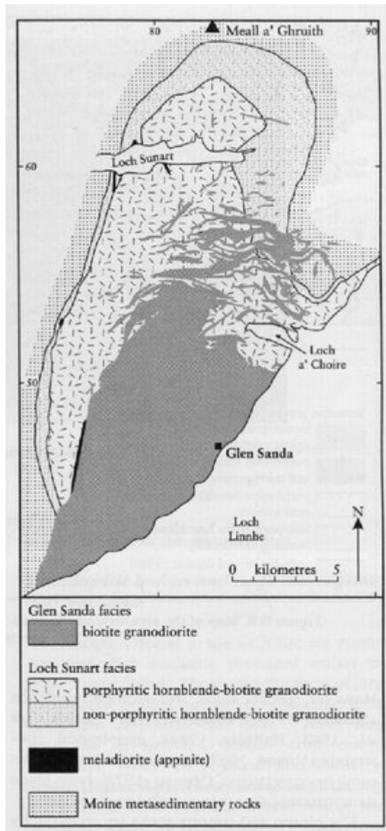
(Figure 8.7) Map showing the distribution of facies within the Strontian pluton, adapted from Sabine (1963).
