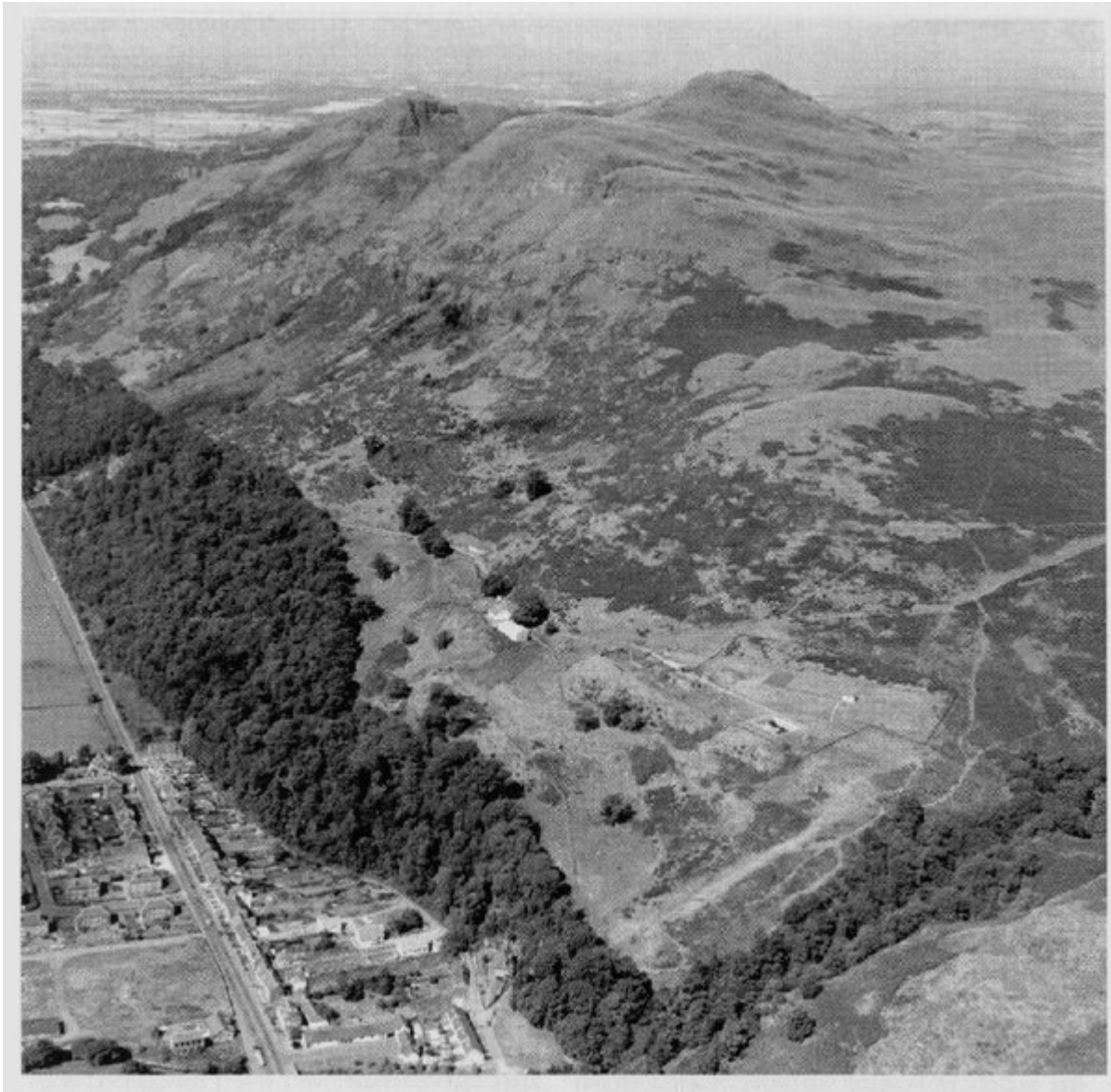
(Figure 9.28) The Ochil Fault scarp above Menstrie. The scarp face exposes a 600 m-thick sequence through the Ochil Volcanic Formation, dipping gently to the north (right). Menstrie Glen is in the bottom right and the prominent summit is Dumyat. (Photo: BGS no. D2066.)
