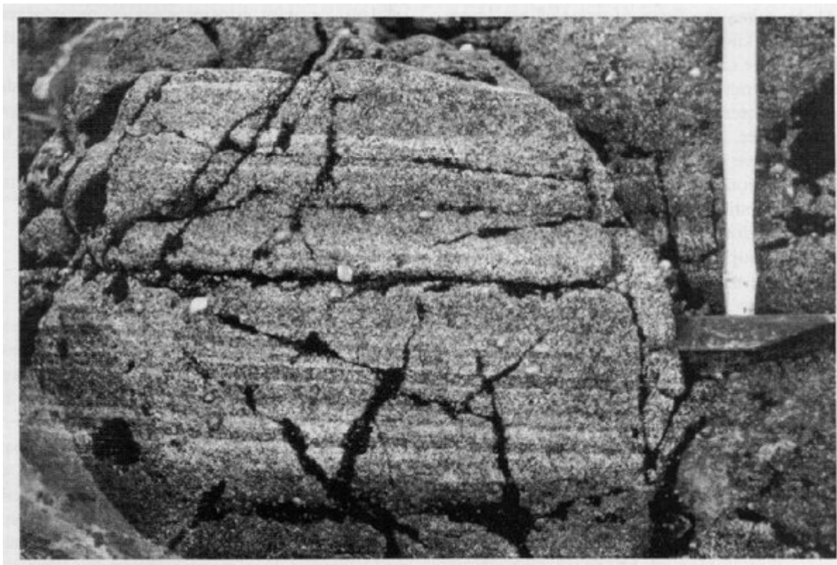
(Figure 2.9) Rhythmic banding in metagabbro [HP 647 077]. (Photo: D. Flinn.)
