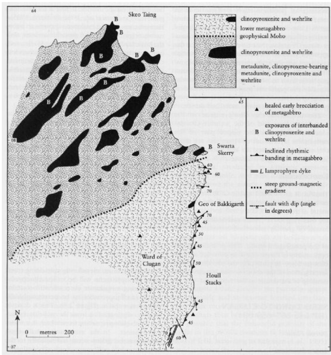
(Figure 2.8) Map of the Skeo Taing area, Unst.
