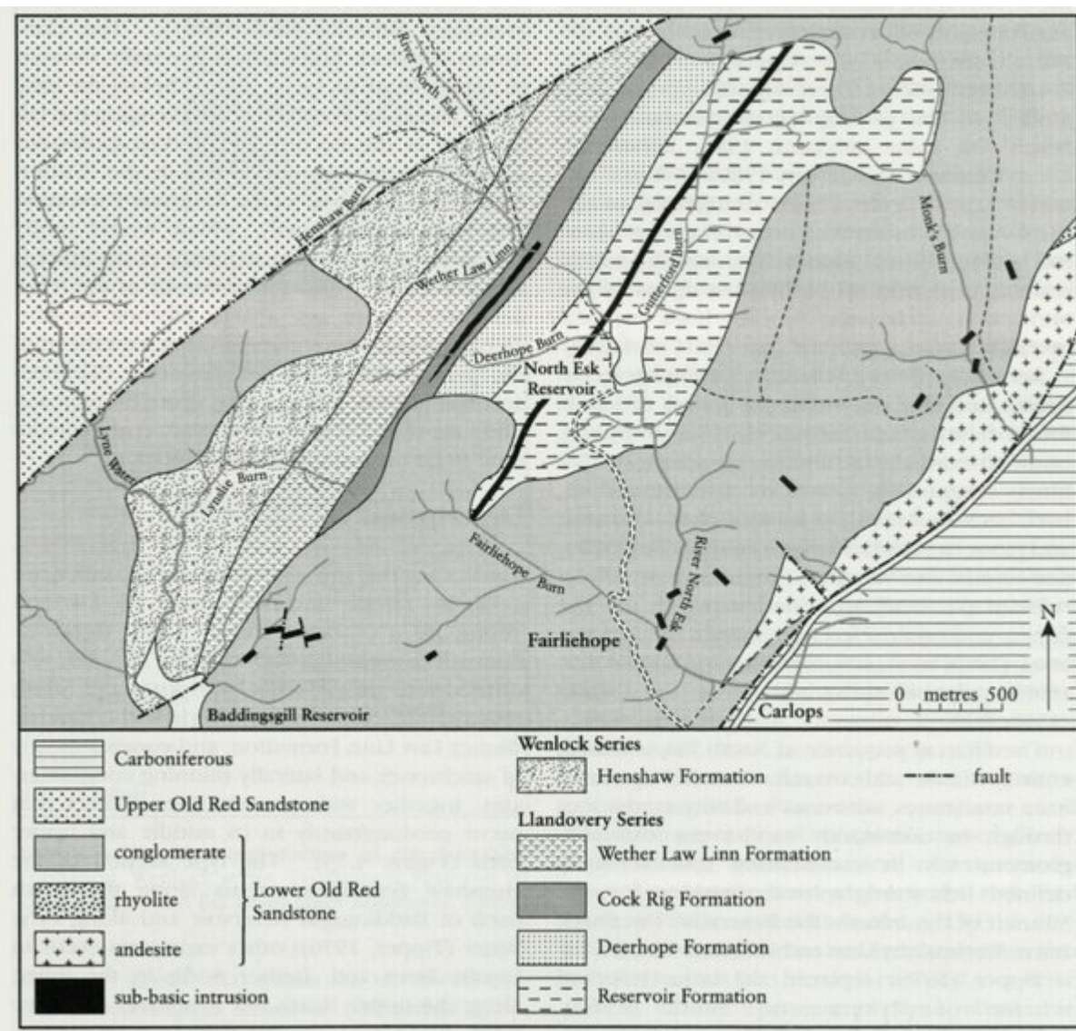
(Figure 4.72) Geology of the North Esk Inlier and location of Lynne Water and Lyslie Burn (after Robertson, 1986, and the British Geological Survey, 1977).
