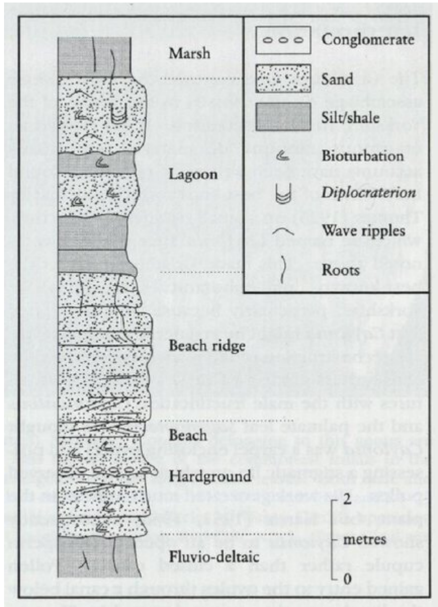
(Figure 3.46) Stratigraphical section through the Cloughton Formation exposed at Cloughton Wyke. (After Livera and Leeder, 1981.)
