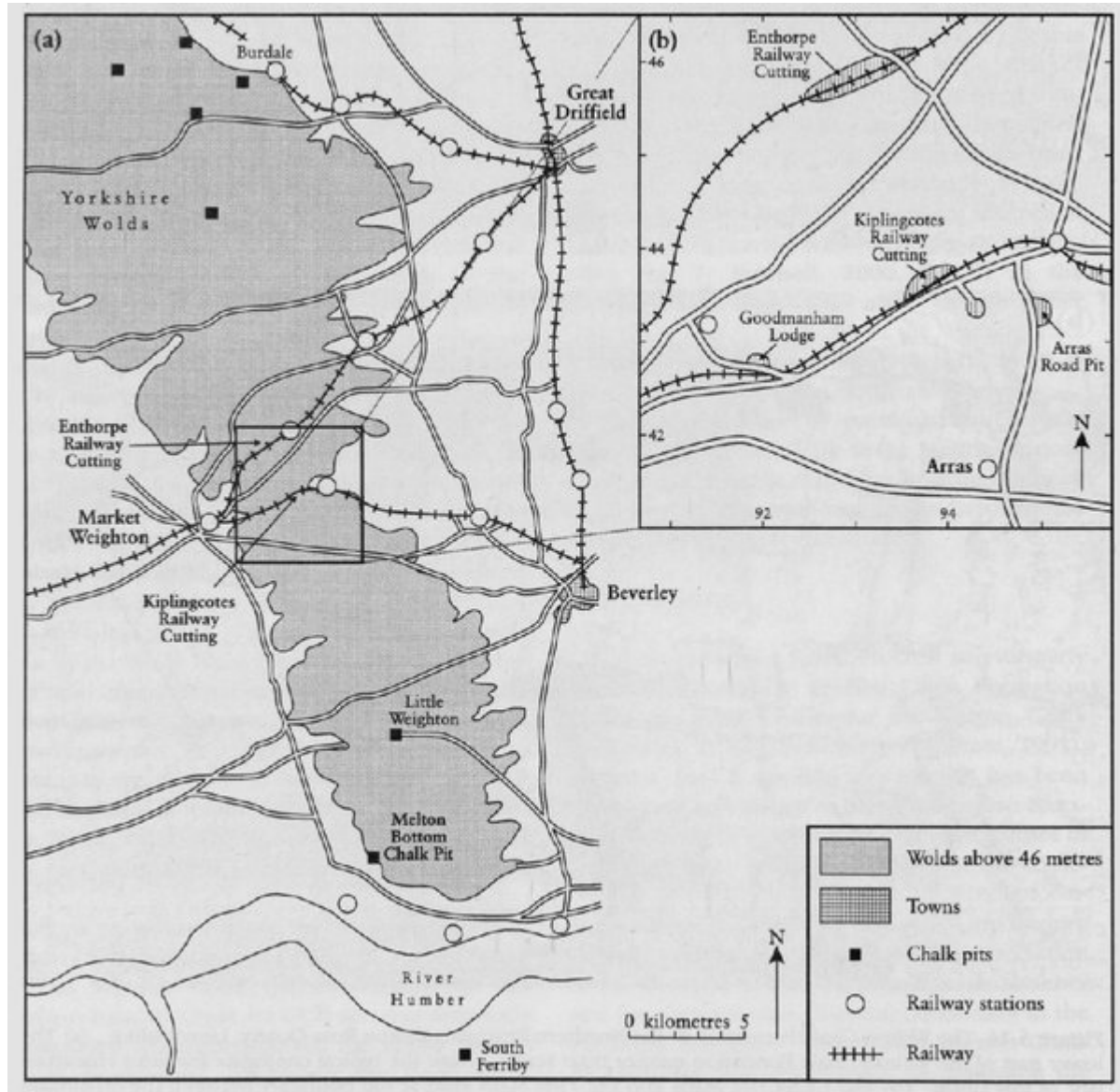
(Figure 5.15) The location of Enthorpe Railway Cutting and other field sections in the Yorkshire Wolds.
