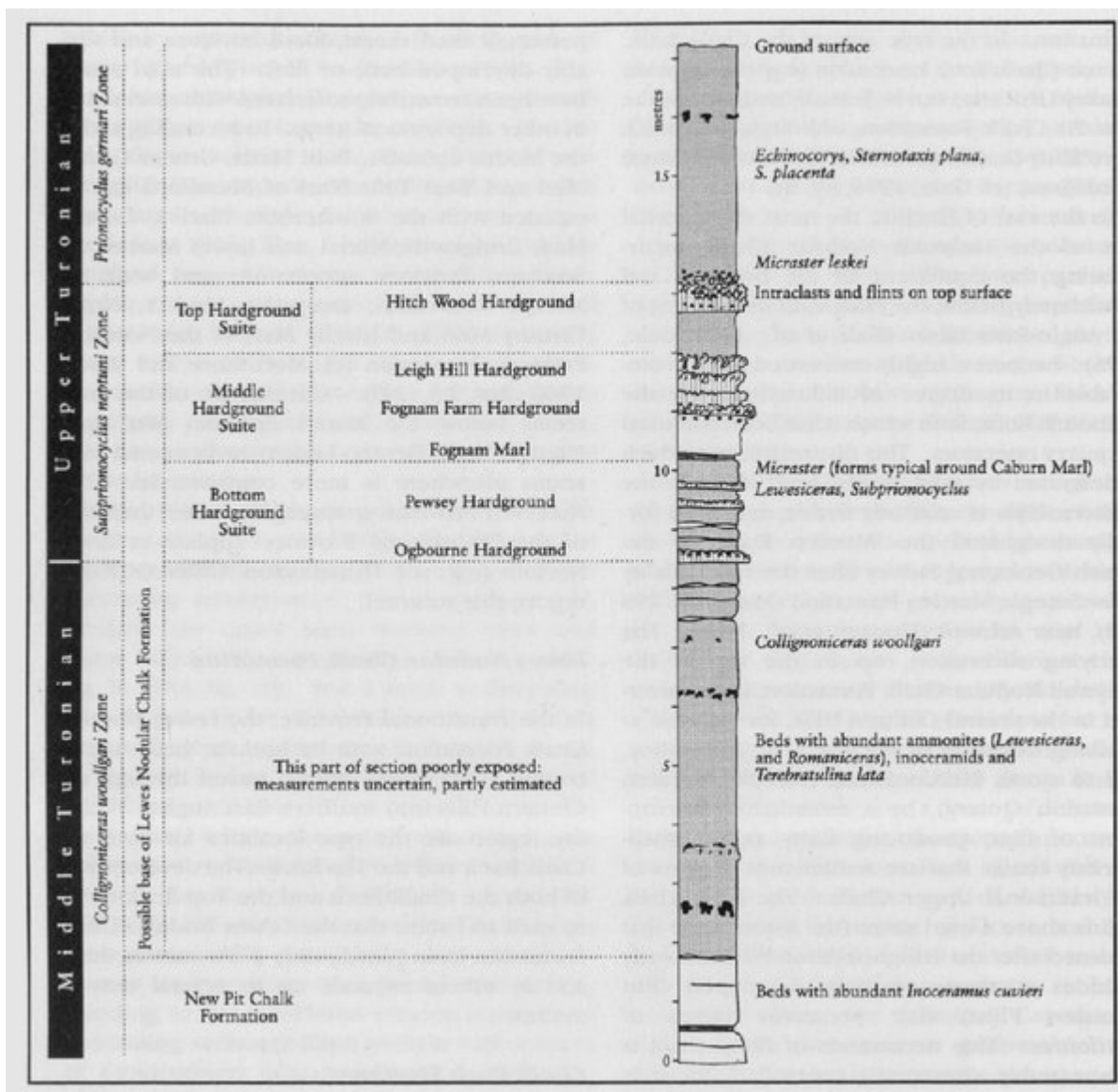
(Figure 4.4) The Chalk succession exposed at Fognani Quarry, a key section for Chalk Rock stratigraphy. Compare with Charnage Down Chalk Pit ((Figure 3.41), Chapter 3) and Kensworth Chalk Pit (Figure 4.21).
