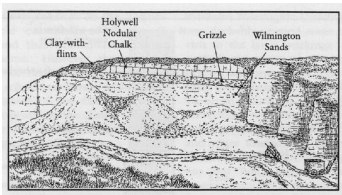
(Figure 3.28) The former section at Reeds Farm Pit, Wilmington, south-east Devon (also known as 'Hutchins Pit' or 'Haynes Lane Pit').
