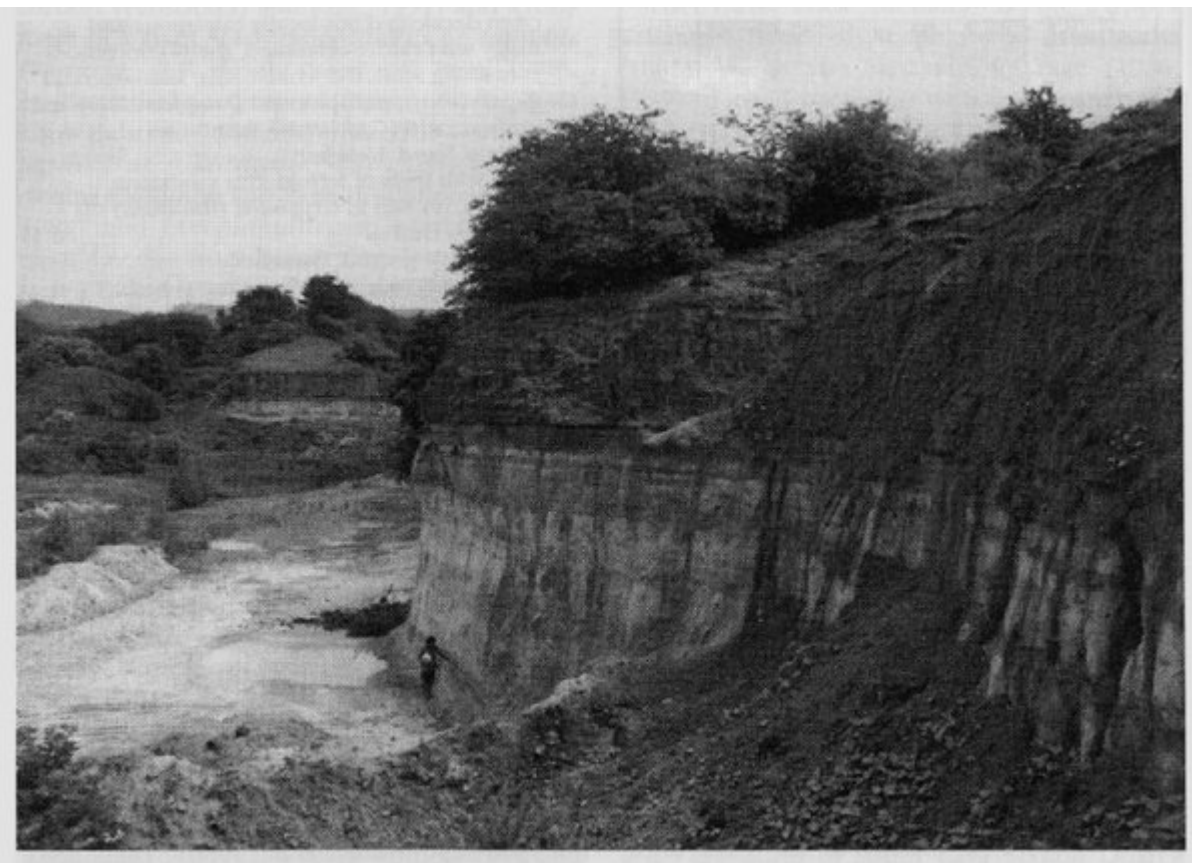
(Figure 4.53) South Cave Station Quarry (part of the Drewton Lane Pits GCR site), showing the pale Kellaways Sand Member overlain by the darker Cave Rock Member. (Photo: M.G. Sumbler.)
