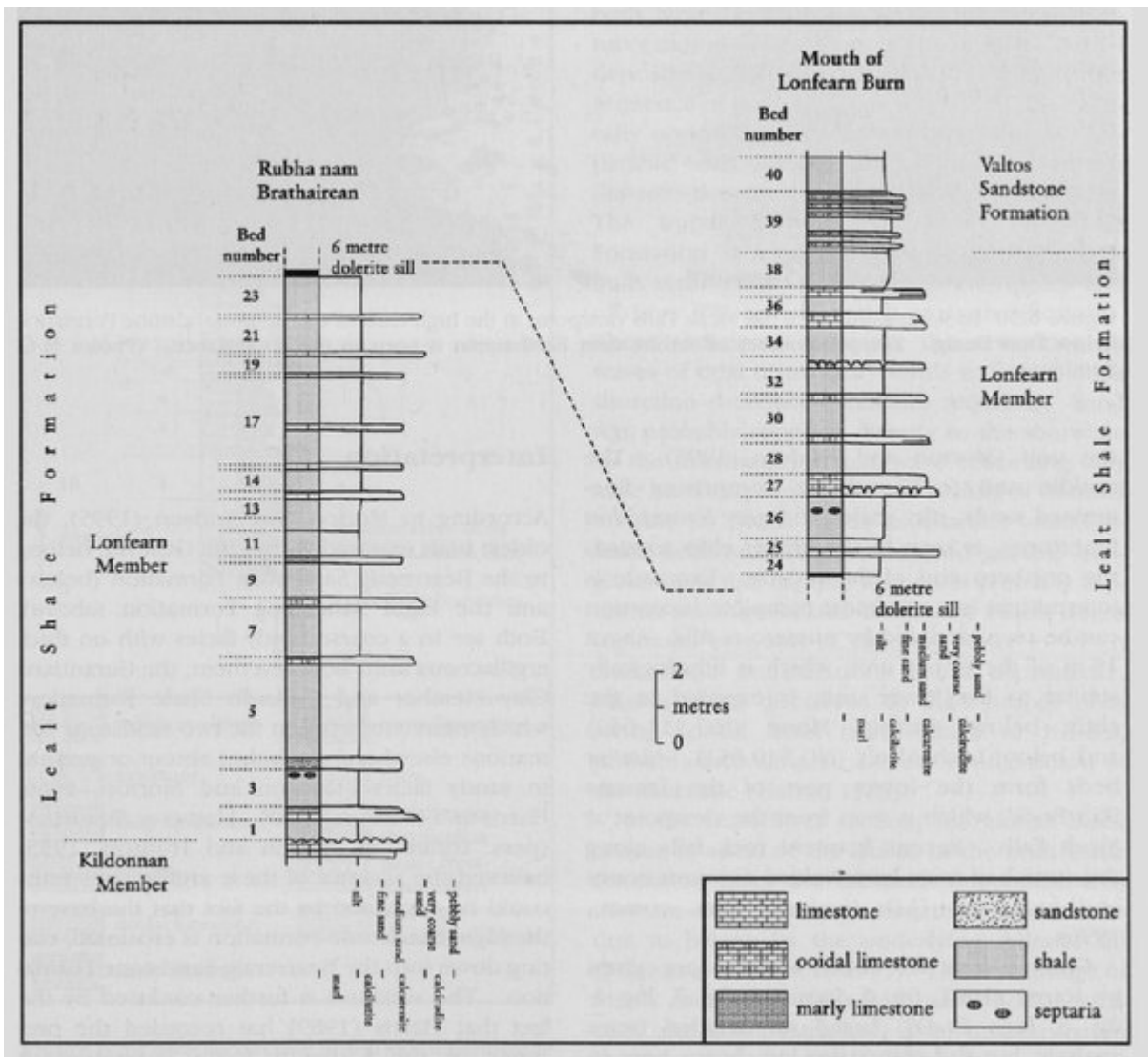
(Figure 6.37) Graphic section of the Lonfearn Member (Lealt Shale Formation) at its type locality (After Harris and Hudson, 1980, fig. 6.) Bed numbers follow Harris and Hudson (1980).
