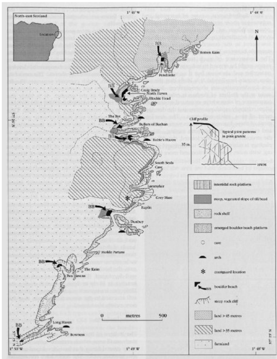
(Figure 3.21) Geomorphological map of the Bulters of Buchan, north-east Scotland. The inset on the right shows the typical cliff profile relative to high-water mark (HWM). Much of the cliff tops are veneered by glacial till. (Modified from unpublished work by W Ritchie.)
