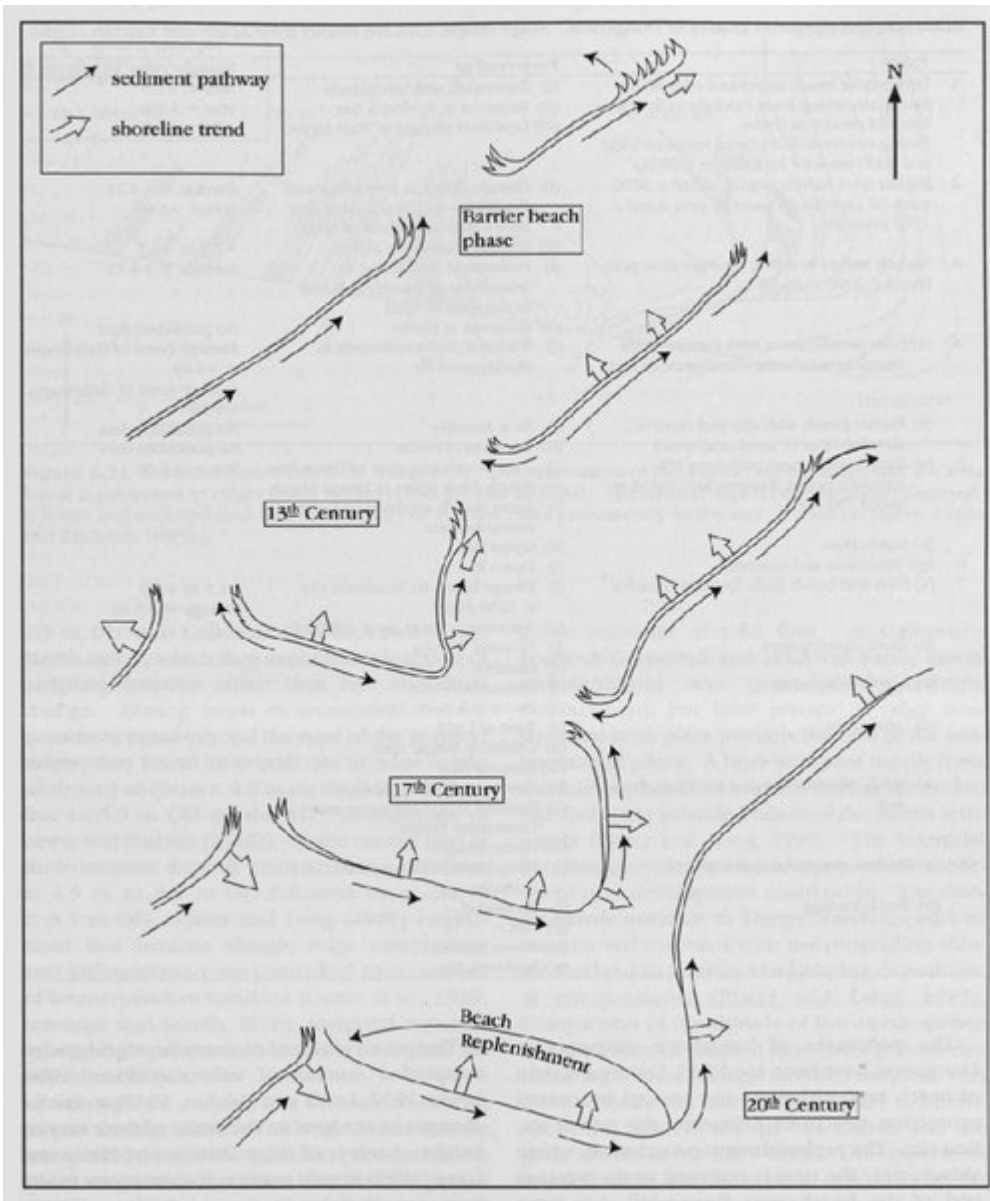
(Figure 6.50) Historical sediment pathways and development at Dungeness. Each schematic map shows the probable sediment movements associated with the erosional and accretional trends in the shoreline.
