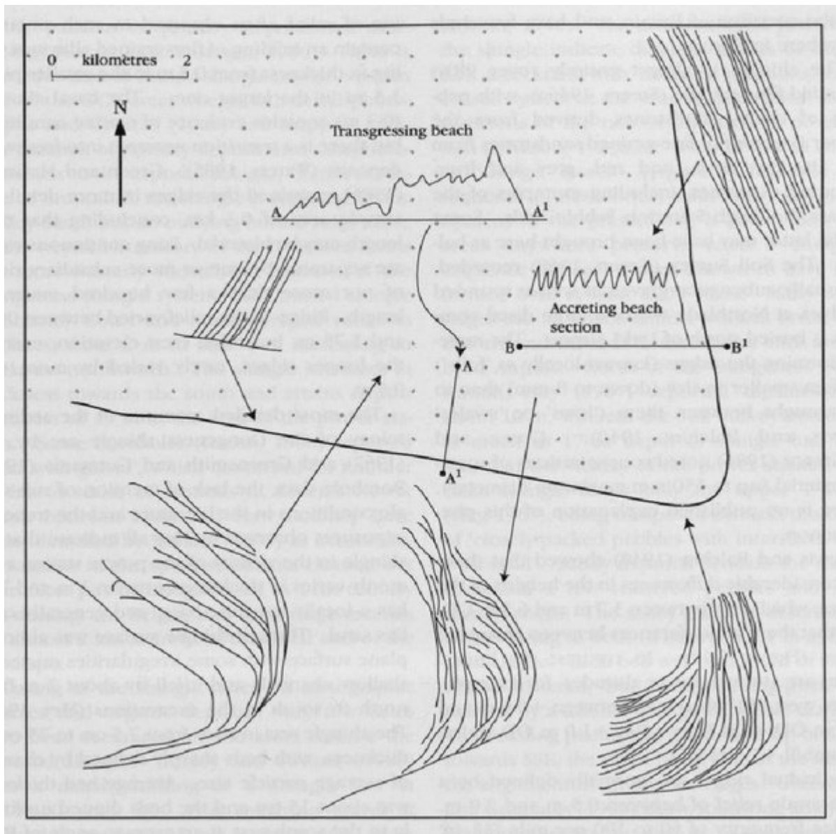
(Figure 6.49) Schematic representation of the characteristic shingle ridge patterns and profiles at Dungeness. The vertical variation in ridge altitude is typically about 3m.
