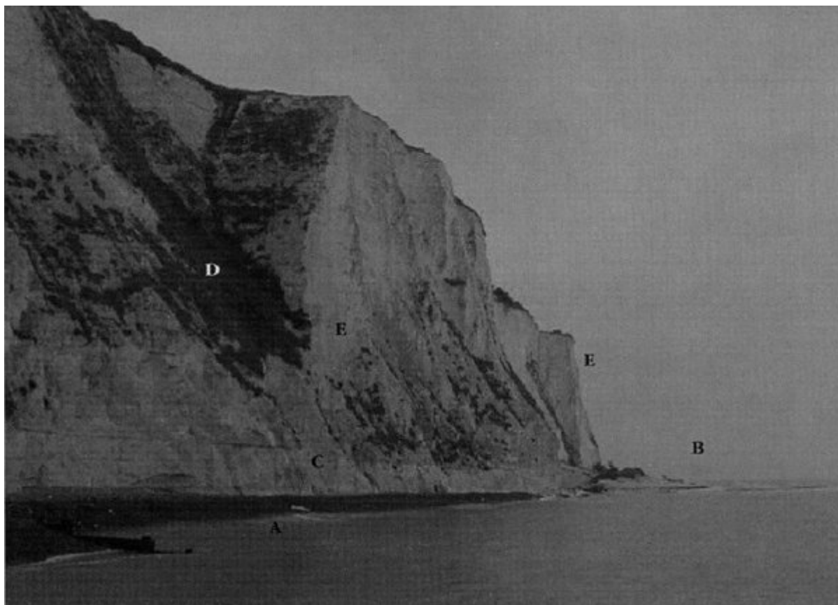
(Figure 4.23) View looking north of St Margaret's Bay, Kingsdown to Dover GCR site. (A) Small, fringing beach of flint, mostly derived from recent cliff falls; movement alongshore is restricted by fall debris; (B) large toe of a slide extending beyond low-water mark; (C) cliff being eroded where previous rock fall has been completely removed; (D) vegetated slope that developed behind a former slide toe and debris; these features then protected cliff-foot bedrock from erosion; (E) typical upper cliff profile above debris slopes. (Photo: V.J. May.)
