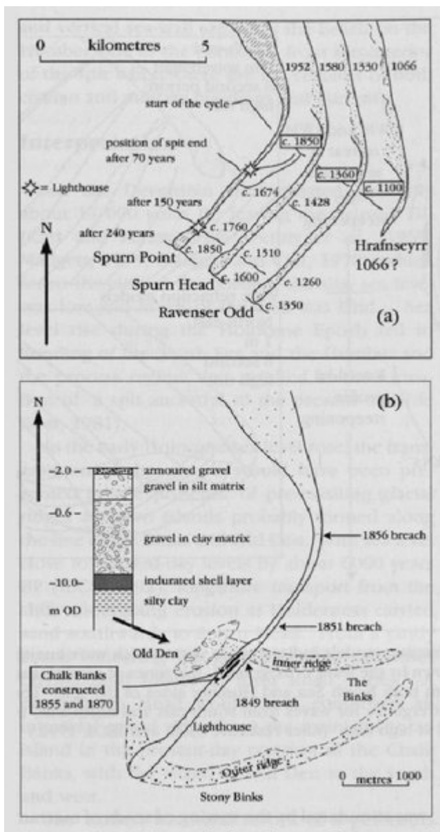
(Figure 8.8) (a) The cyclical evolution of Spurn Head as envisaged by de Boer (1964). Over a period of about 240 years, the spit extends, beginning to develop a spatulate distal end after about 150 years. The neck of the spit is breached and a new cycle of spit growth begins. (b) The key features and 19th century development of Spurn Head. The log shows the sediments underlying Old Den. (After IECS, 1992.)
