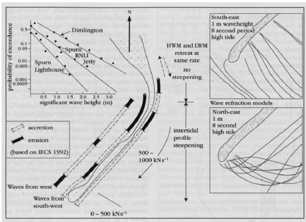
(Figure 8.9) Active processes at Spurn Head. Wave-refraction models indicate areas upon which wave energy concentrates. With waves from different directions (shown by the wave orthogonals), the zones of erosion and accretion change, giving rise to possible breaching from both North Sea and Humber sides of the spit. The wave-refraction models show wave convergence and divergence for waves from south-east and north-east, in both cases for waves 1 m-high, of period 8 seconds and at high tide. (After Halcrow, 1988; and IECS, 1992.)
