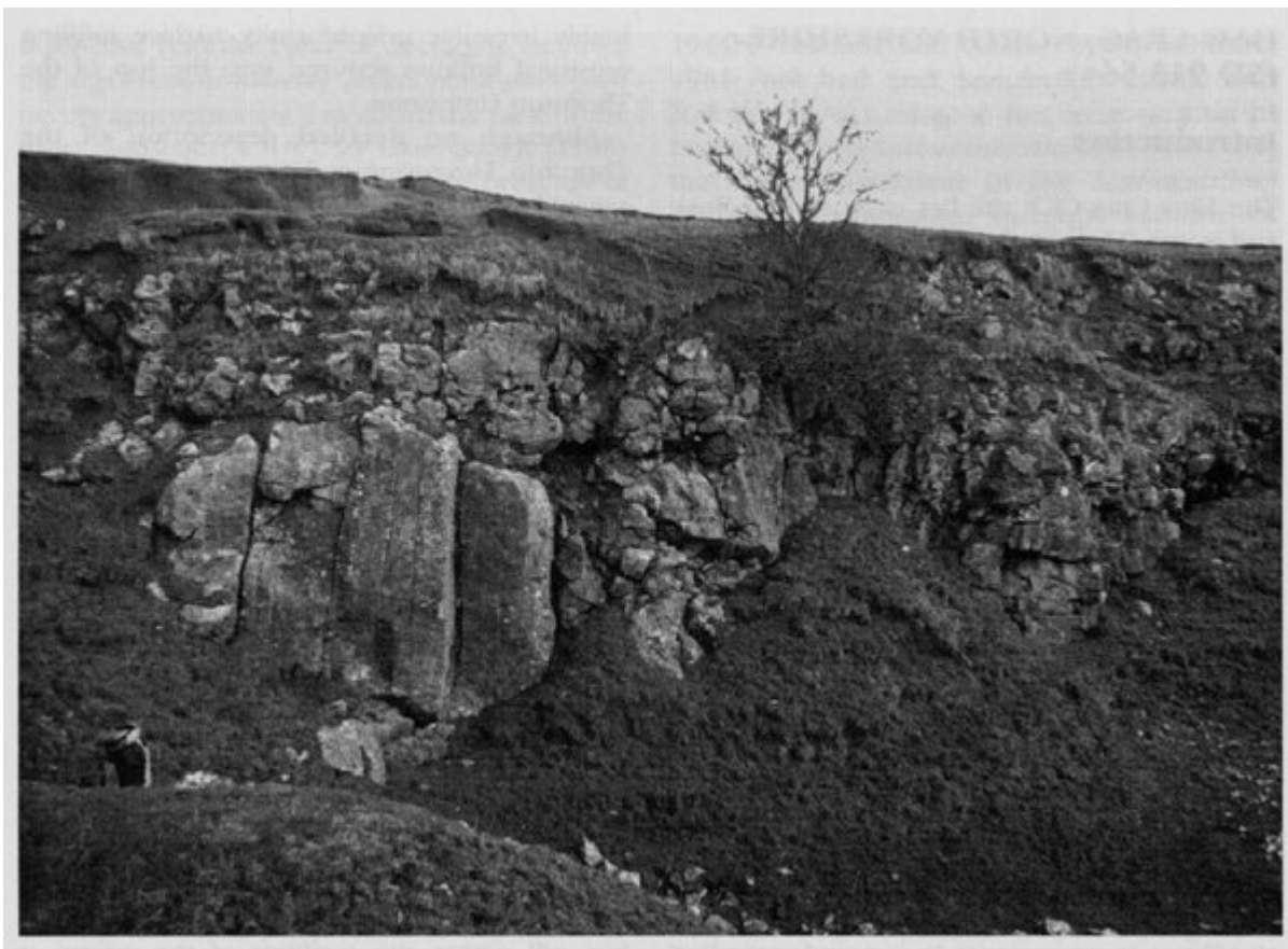
(Figure 6.21) Exposure of the Arundian debris-flow deposit (the Haw Crag Boulder Bed) in the Hodder Mudstone Formation at Haw Crag Quarry, Bell Busk. Note that the prominent block at the foot of the crag (a boulder of the Hetton Beck Limestone Member) is approximately 5 m in diameter. (Photo: P.J. Cossey.)
