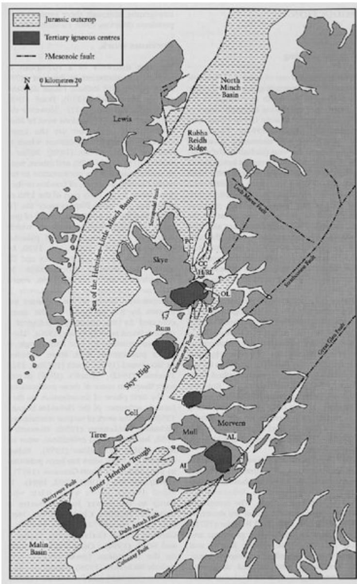
(Figure 8.1) Map of the Jurassic (including Lias Group) outcrop in western Scotland, showing the locations of the GCR sites, indicated in bold, as follows: AI — Aird na h-Iolair; AL — Allt Leacach; B — Boreraig to Cam Dearg; CC — Cadha Carnach; H — Hallaig; OL — Ob Lusa to Ardnish; PC — Prince Charles' Cave to Holm; RL — Rubha na Leac. After Hesselbo et al. (1998).
