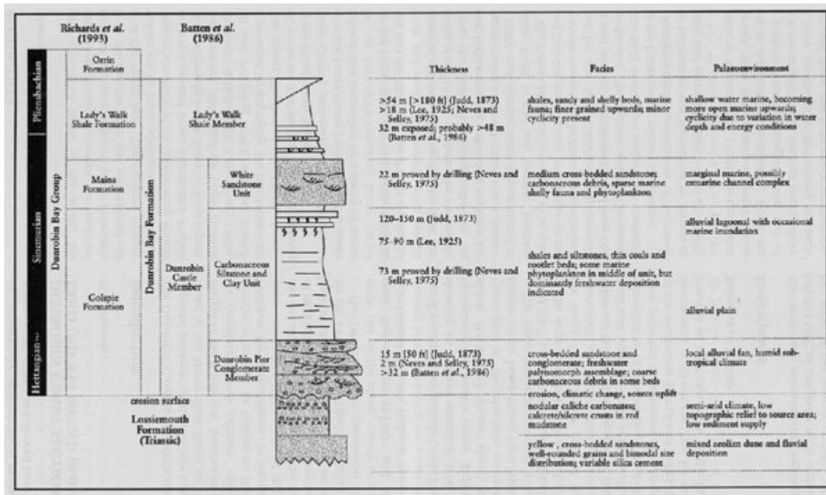
(Figure 7.1) Summary stratigraphy and interpretation of the succession at Dunrobin. After Batten et al. (1986).
