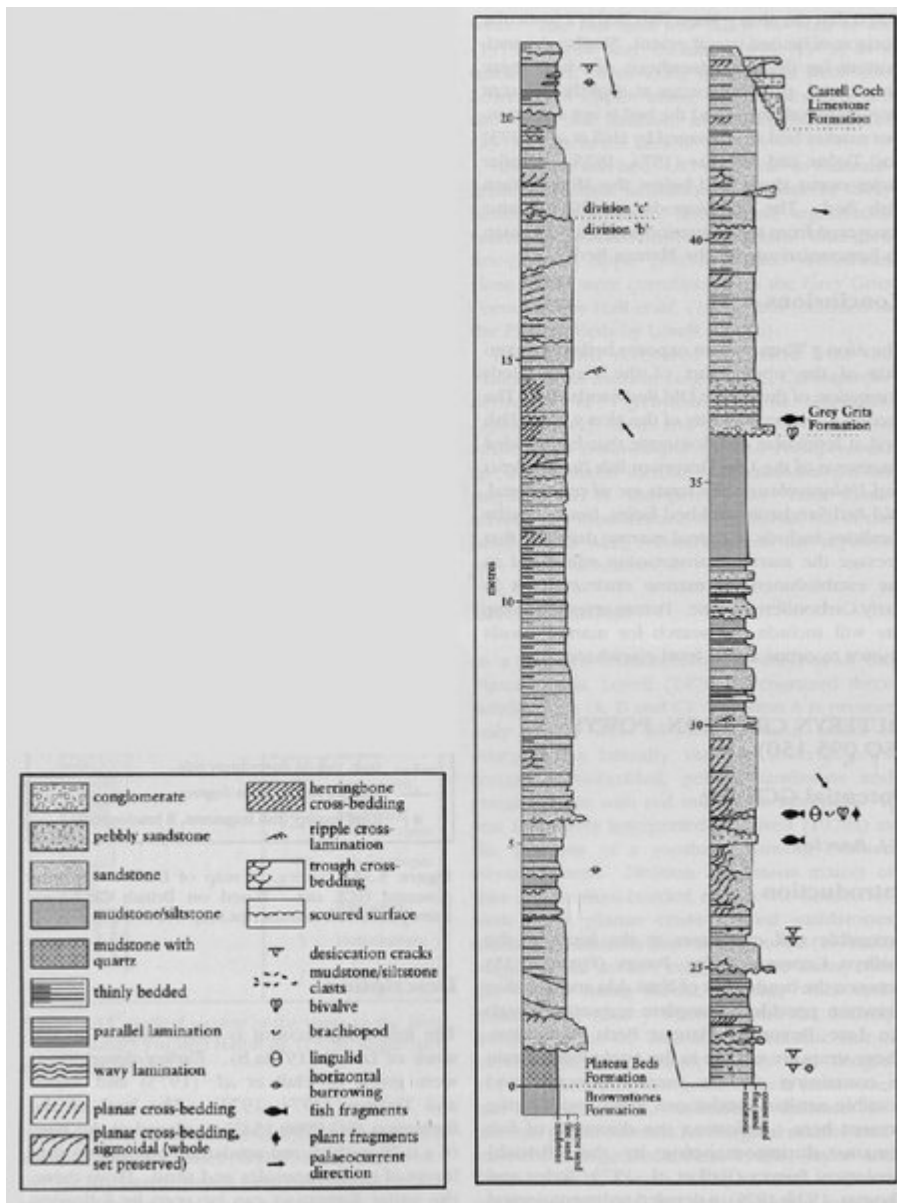
(Figure 5.36) Vertical section of the strata at Duffryn Cawnon. After Lovell (1978a,b).
