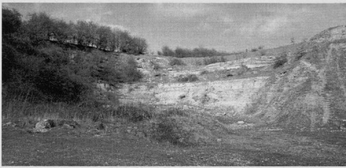
(Figure 2.11) General view of the disused Kirtlington Old Cement Works quarry, Oxfordshire. Exposures of White Limestone, Forest Marble and Cornbrash formations. (Photo: Dave Evans.)
