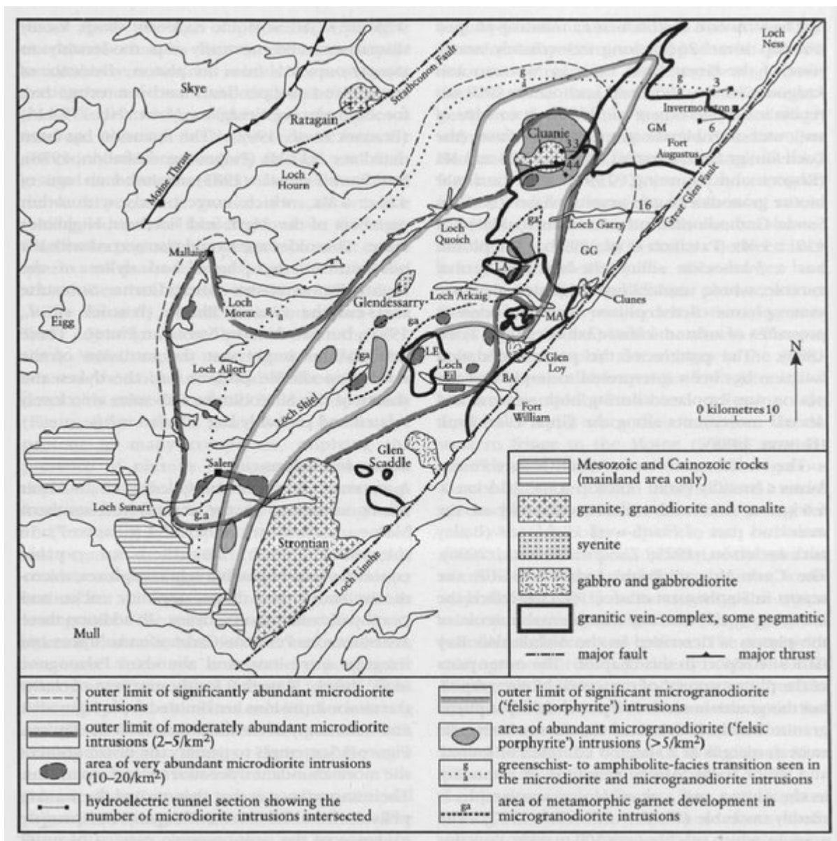
(Figure 8.5) Map showing the Caledonian major and minor intrusions. Granitic vein-complexes: Ba — Banavie; GG — Glen Garry; GM — Glen Moriston; LA — Loch Arkaiq; LE — Loch Eil; MA — Maine.
