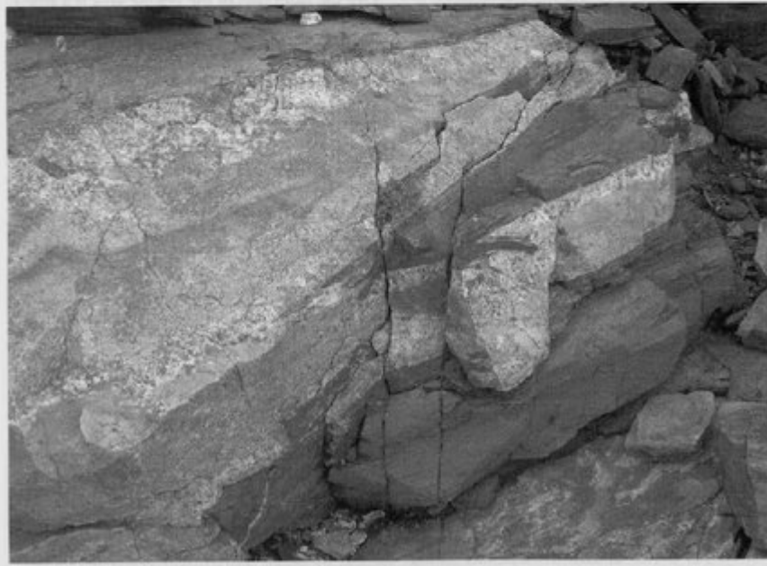
(Figure 7.12) (a) View across Tremearne Par and Megilligar Rocks towards Wheal Trewavas copper mine. (b) The contact between the pegmatite and the killas, Tremearne Par. (Photos: H. Townley, Natural England.)
