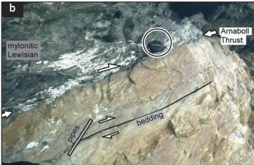
The classic location (2C) of the Arnaboll Thrust and of Lapworth's (1883) mylonites: (a) general aspect of the thrust, carrying Lewisian gneisses onto Pipe Rock; hammer (circled) for scale (b) detail of the Arnaboll Thrust, showing deflected Skolithos (pipes) that indicate the sense of shear (top to WNW); scale from lens cap (circled)
