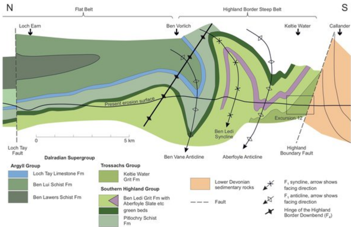
(Figure S.2) Cross-section of the Tay Nappe from Callander due north to Loch Eam, showing the Flat Belt, Highland Border Downbend ( F_4 ) and major downward-facing F_1 folds in the Highland Border Steep Belt (adapted from Tanner et al, 2013, fig. 13).
