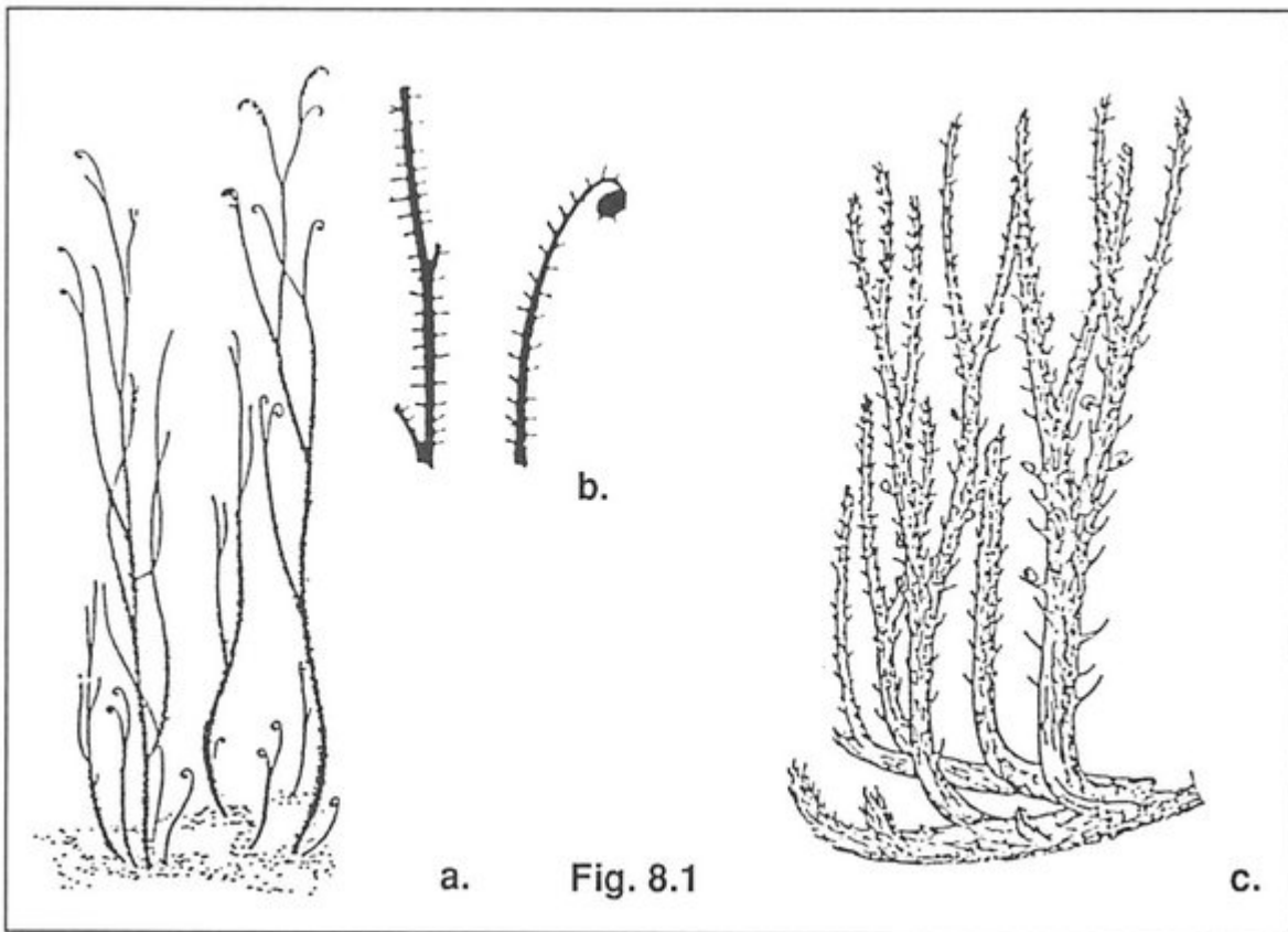
(Figure 8.1) Plants from the Lower Old Red Sandstone of Auchensail Quarry. a. Sawdonia ornata (reconstruction, \times 0.1 ), b. Sawdonia ornata (stems, \times 0.05 ), c. Drepanophycus spinæformis (reconstruction, \times 0.15 ) [Redrawn after Rolfe, 1976]
