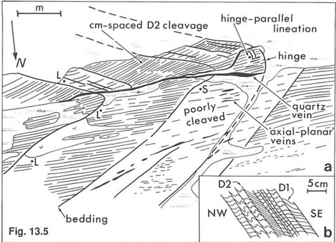
(Figure 13.5) a) Down-plunge true-scaled drawing of a D_2 fold at Locality 2. L, location of bedding-cleavage intersection line; S, possible stretching lineation. b) Close-up view of the D_2 cleavage showing the deformed D_1 cleavage.
