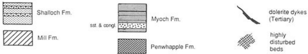
(Figure 30.3) Detailed geological map of the foreshore at Port Cardloch.
