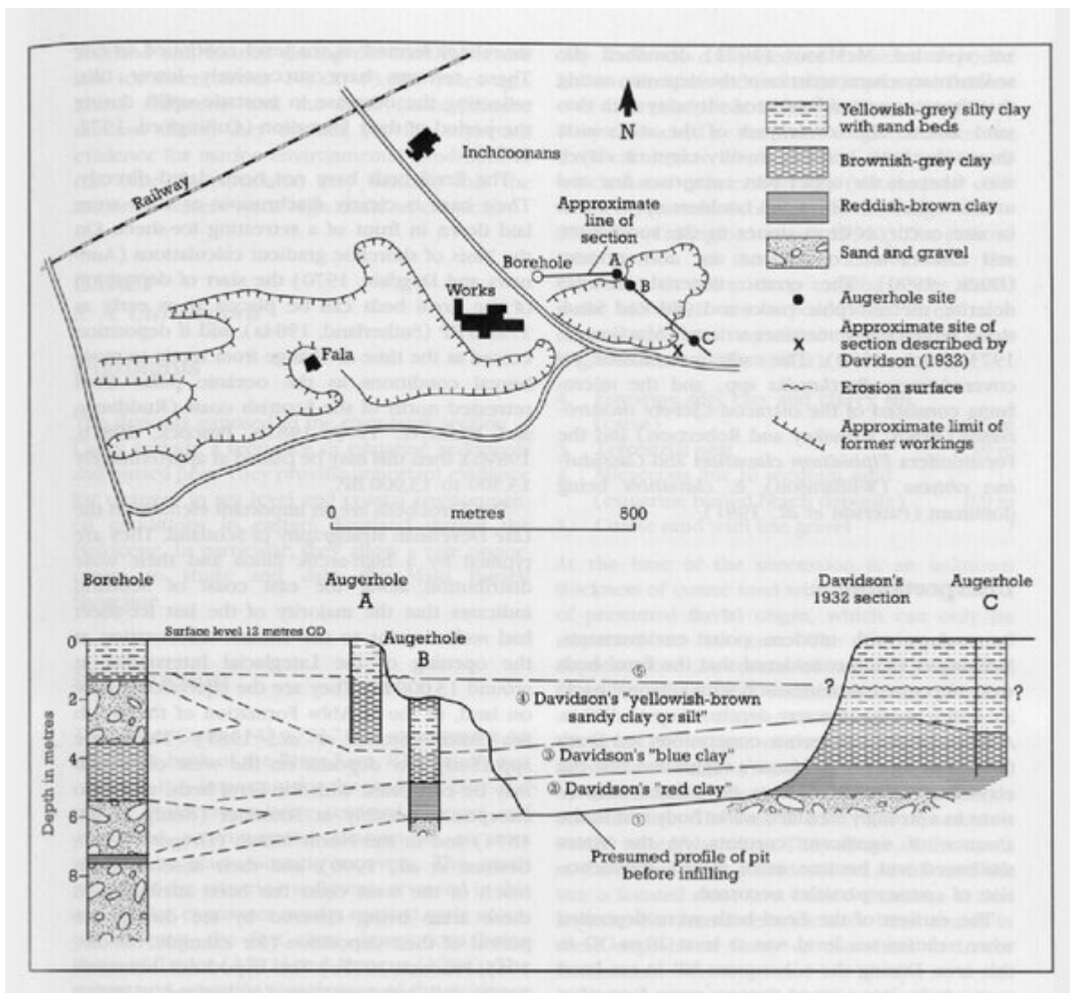
(Figure 15.2) Inferred stratigraphy of the Errol beds at Inchcoonans claypit (from Paterson et al., 1981).
