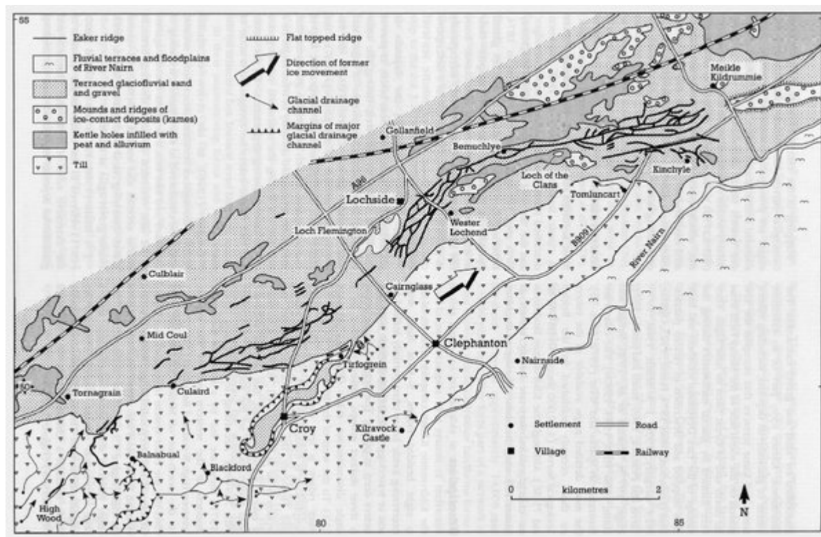
(Figure 7.11) Geomorphology of the Kildrummie Kames esker system between High Wood and Meikle Kildrummie (from mapping by C. A. Auton for the British Geological Survey 1:50,000 Geological Sheet 84W (Fortrose), in press).
