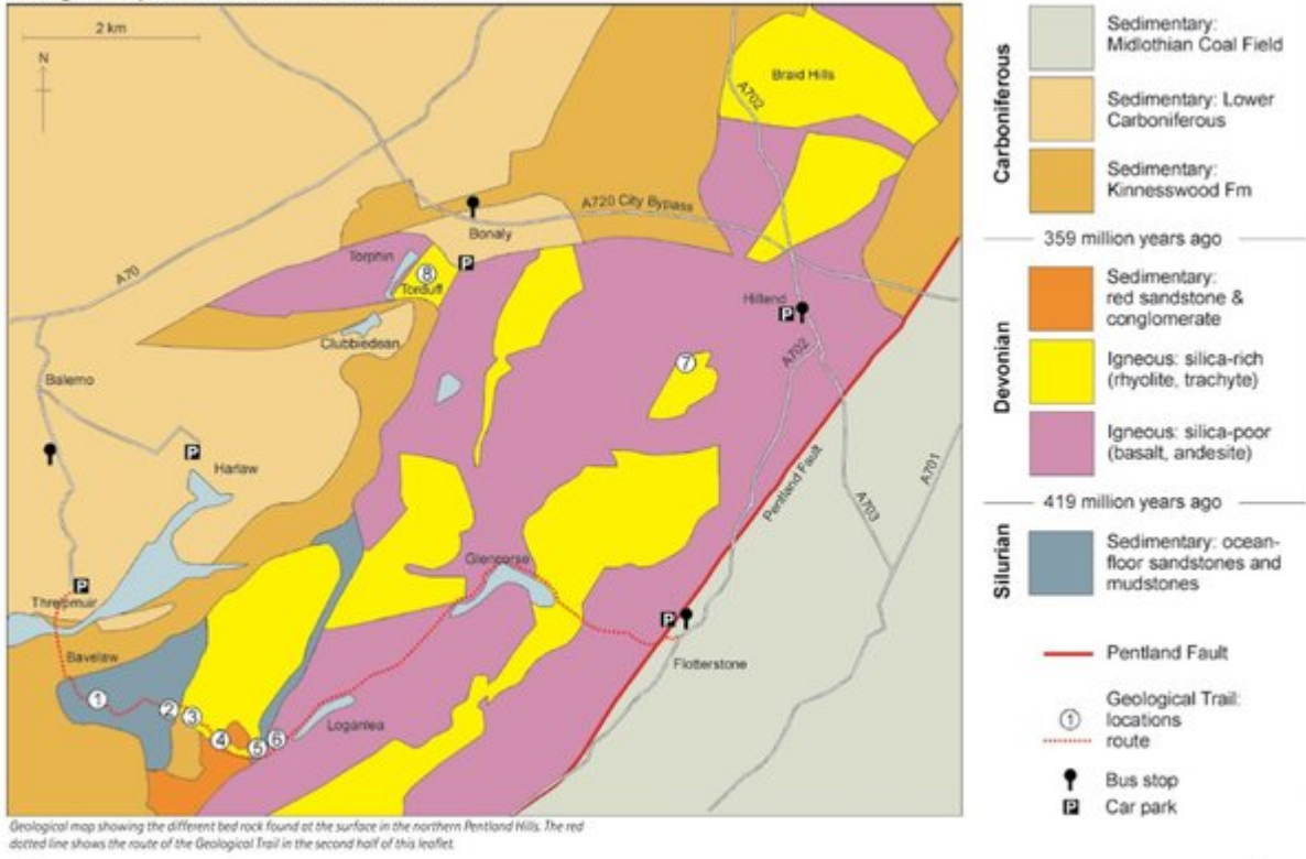
Geological map of the northern Pentland Hills
