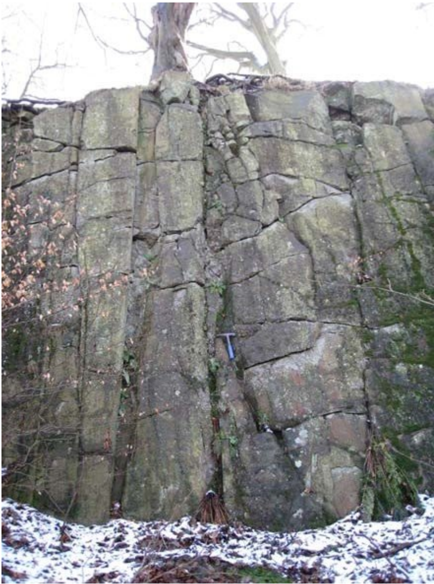
(Photo 13) Well-developed sub-vertical columnar jointing in the quartz-microgabbro. Looking SSE.
