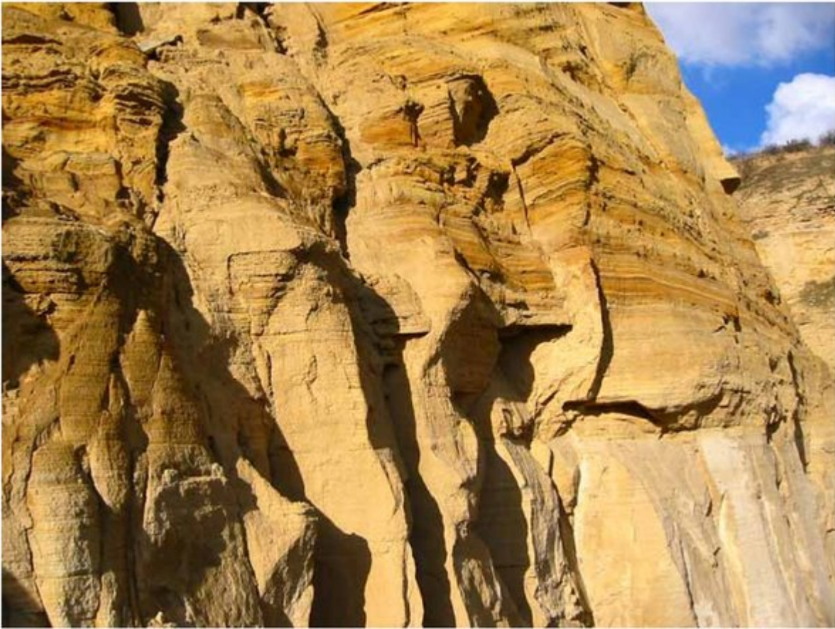
(Plate 24) Cross-bedding in Permian Yellow Sands Formation at Crime Rigg Quarry.
