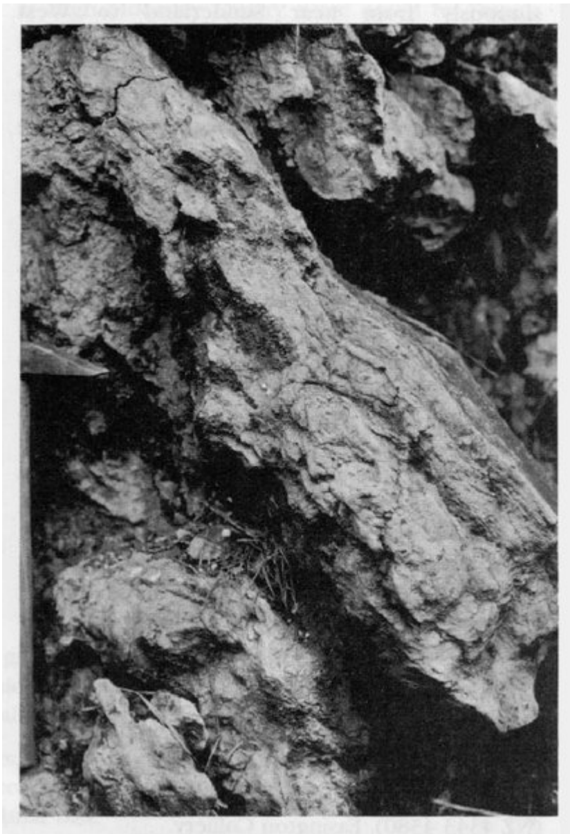
(Figure 3.43) Laminae algal bindstone sheets with high primary east-northeastwards dip, in reef boundstone of the Ford Formation near the north-east end of Stony Cut, Cold Hesledon. The sheets are thought to mark the temporary position of the upper part of the reef foreslope and grade upwards into the reef-crest and reef-flat dolomite. Hammer: 0.33 m. (Photo: D.B. Smith.)
