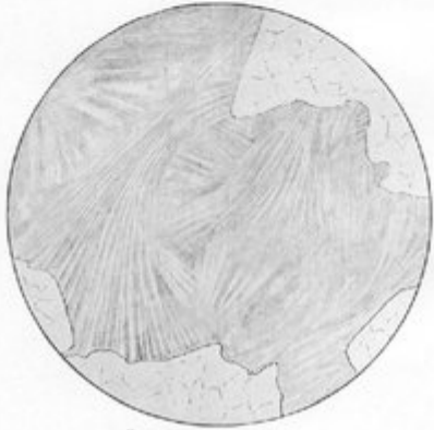
FIG. 4. New-formed felspar.
