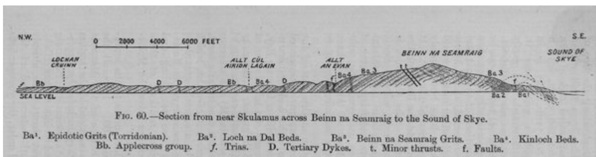
(Figure 60) Section from near Skulamus across Beinn na Seamraig to the Sound of Skye. Ba¹. Epidotic Grits (Torridonian). Ba². Loch na Dal Beds. Ba³. Beinn na Seamraig Grits. Ba⁴. Kinloch Beds. Bb. Applecross group. f. Trias. D. Tertiary Dykes. t. Minor thrusts. f. Faults.
