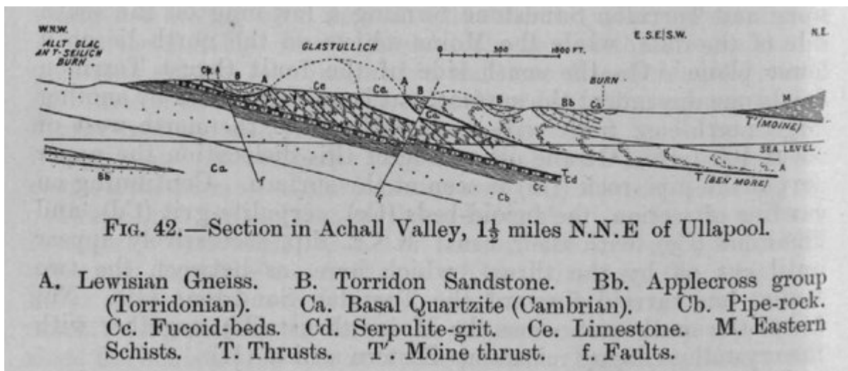
(Figure 42) Section in Achall Valley, 1½ miles N.N.E of Ullapool. A. Lewisian Gneiss. B. Torridon Sandstone. Bb. Applecross group (Torridonian). Ca. Basal Quartzite (Cambrian). Cb. Pipe-rock. Cc. Fucoid-beds. Cd. Serpulite-grit. Ce. Limestone. M. Eastern Schists. T. Thrusts. T'. Moine thrust. f. Faults.
