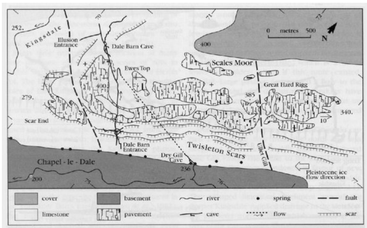
(Figure 2.11) Geological map of Scales Moor. The limestone is the Great Scar Limestone, including the Hawes Limestone. Cover rocks are mainly clastic units in the Wensleydale Group. Basement rocks are Palaeozoic slates and greywackes. Only the larger areas of pavement are marked, and there are thin strips of pavement along the crest of nearly all the scars. Dale Barn Cave lies close to the base of the limestone, about 150 m below the main limestone pavements (cave survey from Northern Cave Club).
